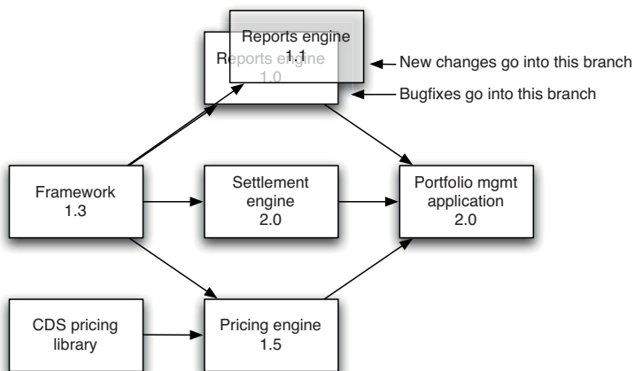
Figure 13.6 Branching components
